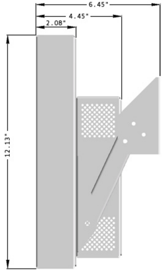
Wallmount Position
